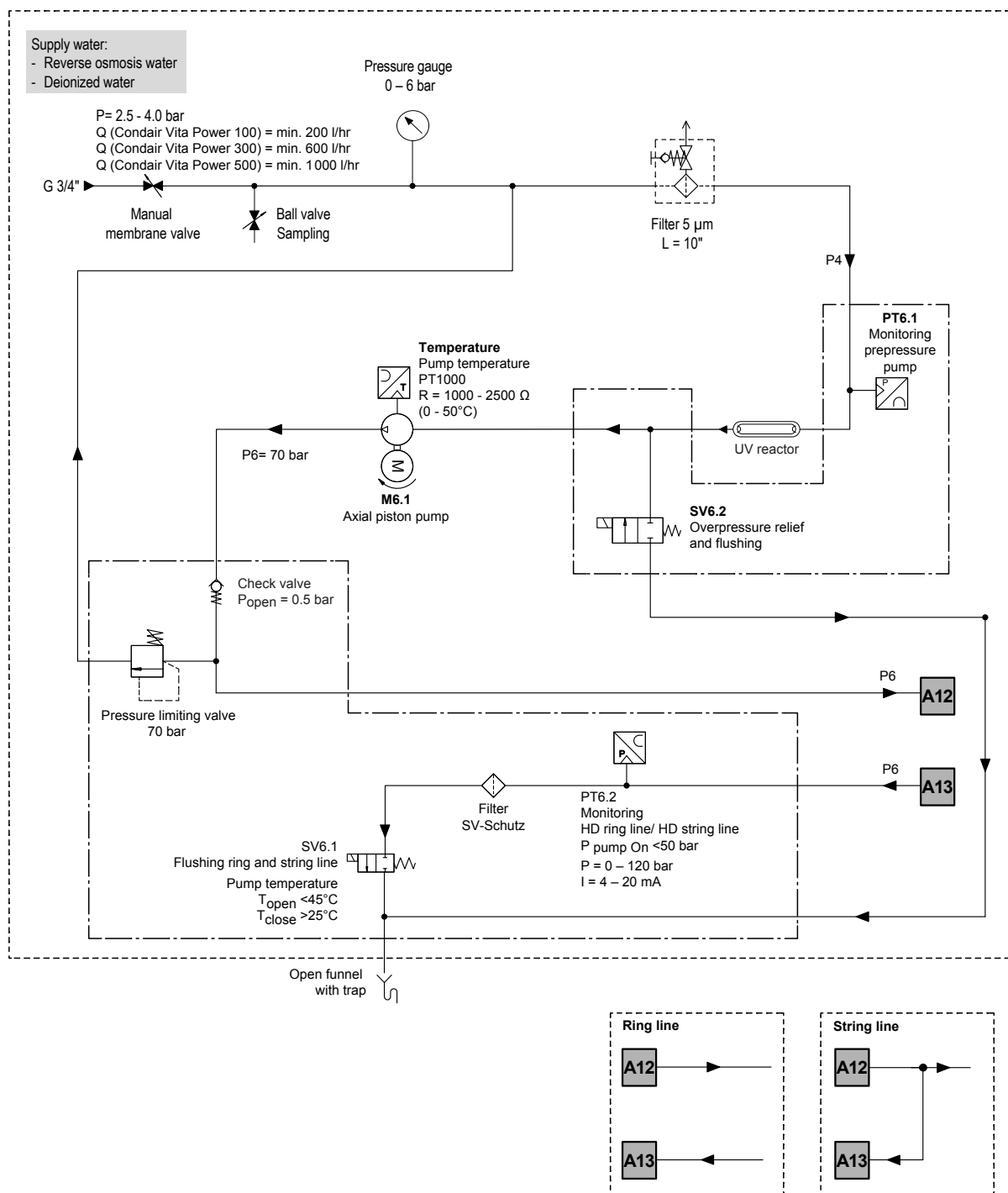
Fig. 26: Hydraulic diagram Condair Vita Power UV-HP
