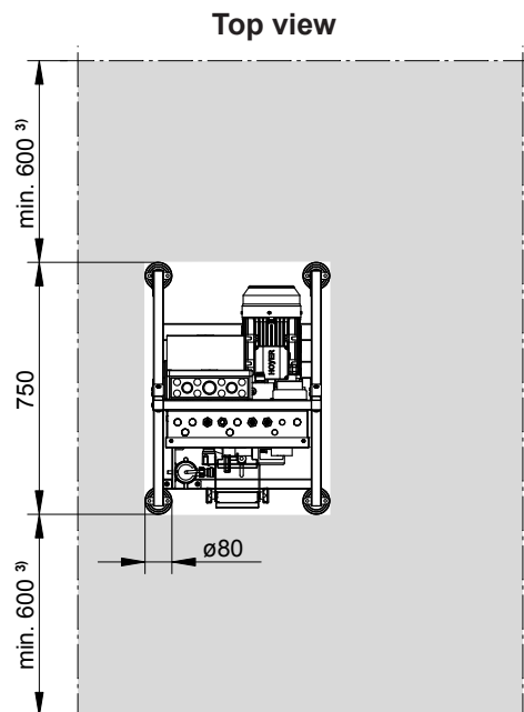
Fig. 7: System dimensions / recommended distances Vita Power RO-UV-HP (dimensions in mm)
