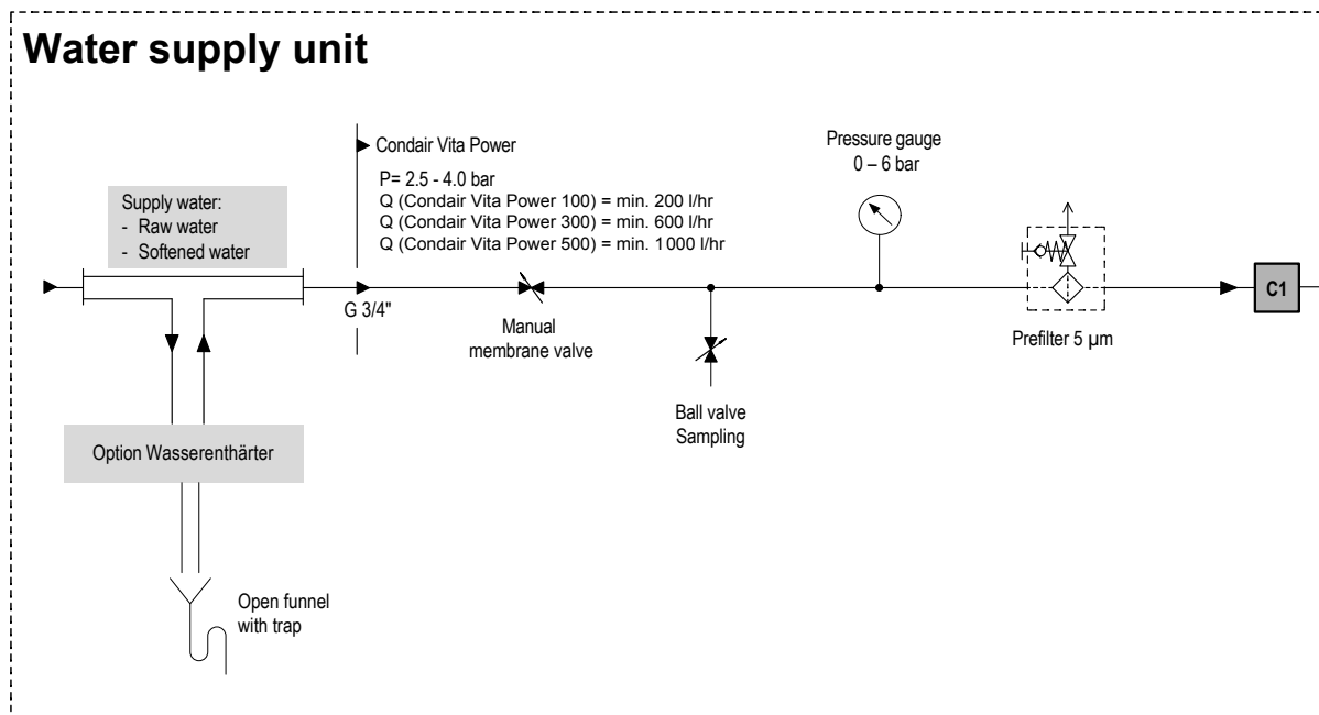
Fig. 19: Hydraulic diagram water supply
