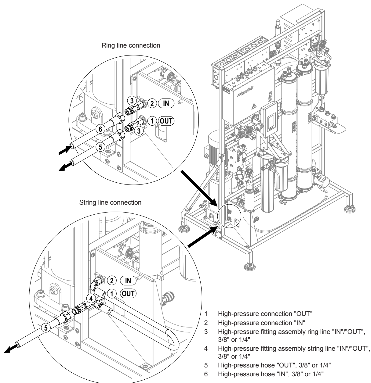
Fig. 15: Connecting the high pressure lines to the Condair Vita Power (image shows Condair Vita Power RO-DI-CO-UV-HP 500 l/hr)
