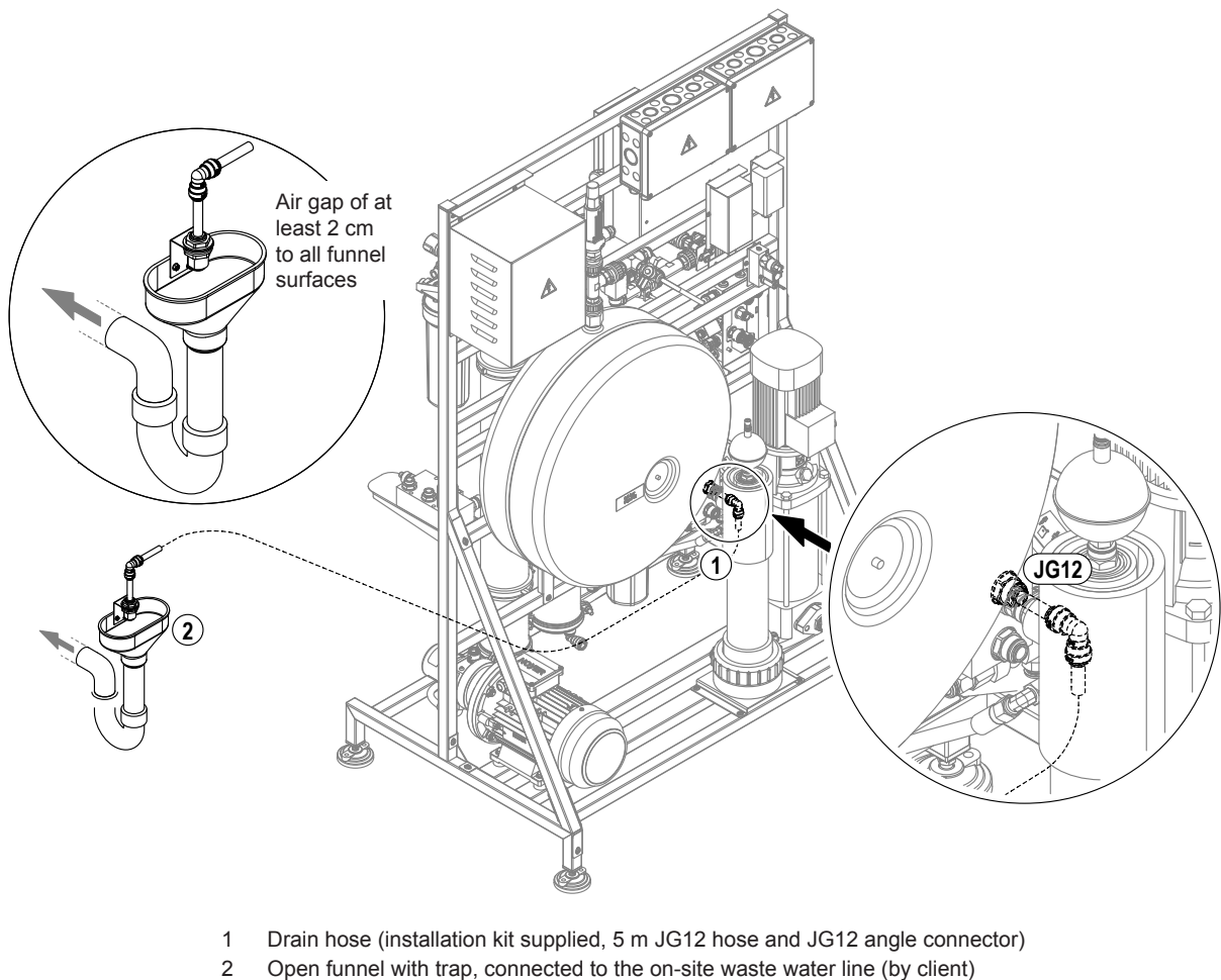
Fig. 14: Connecting the drain line to the Condair Vita Power (image shows Condair Vita Power RO-DI-CO-UV-HP 500 l/hr, tank side)
