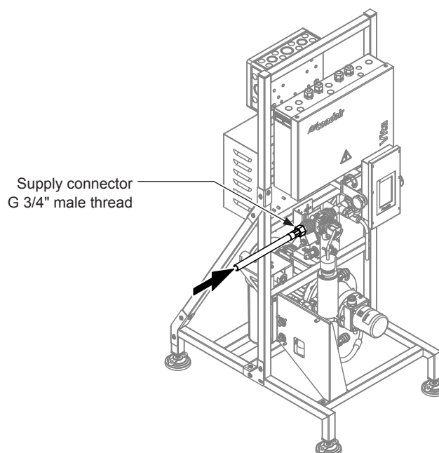
Fig. 11: Water supply connection (image shows Condair Vita Power UV-HP 500 l/h)
