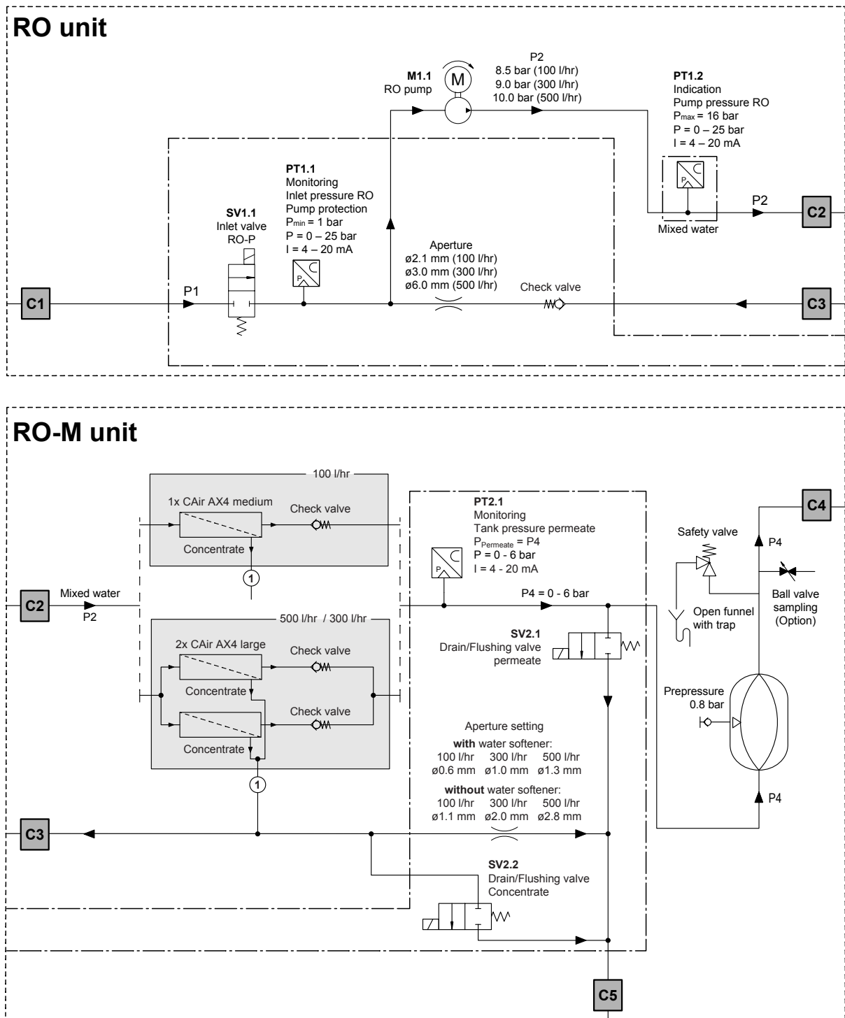
Fig. 24: Hydraulic diagram RO-P / RO-M unit
