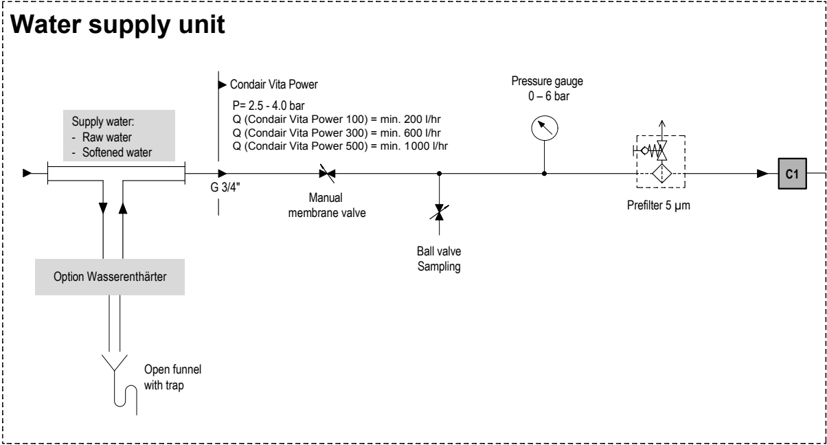
Fig. 23: Hydraulic diagram water supply
