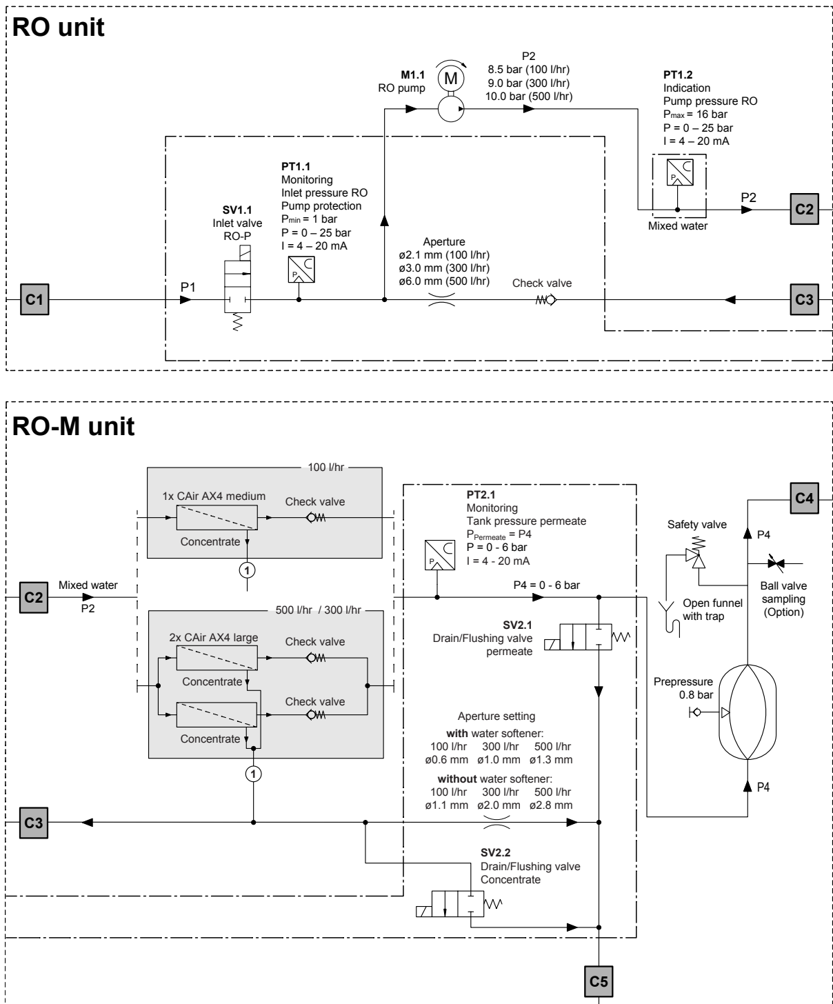
Fig. 20: Hydraulic diagram RO / RO-M unit
