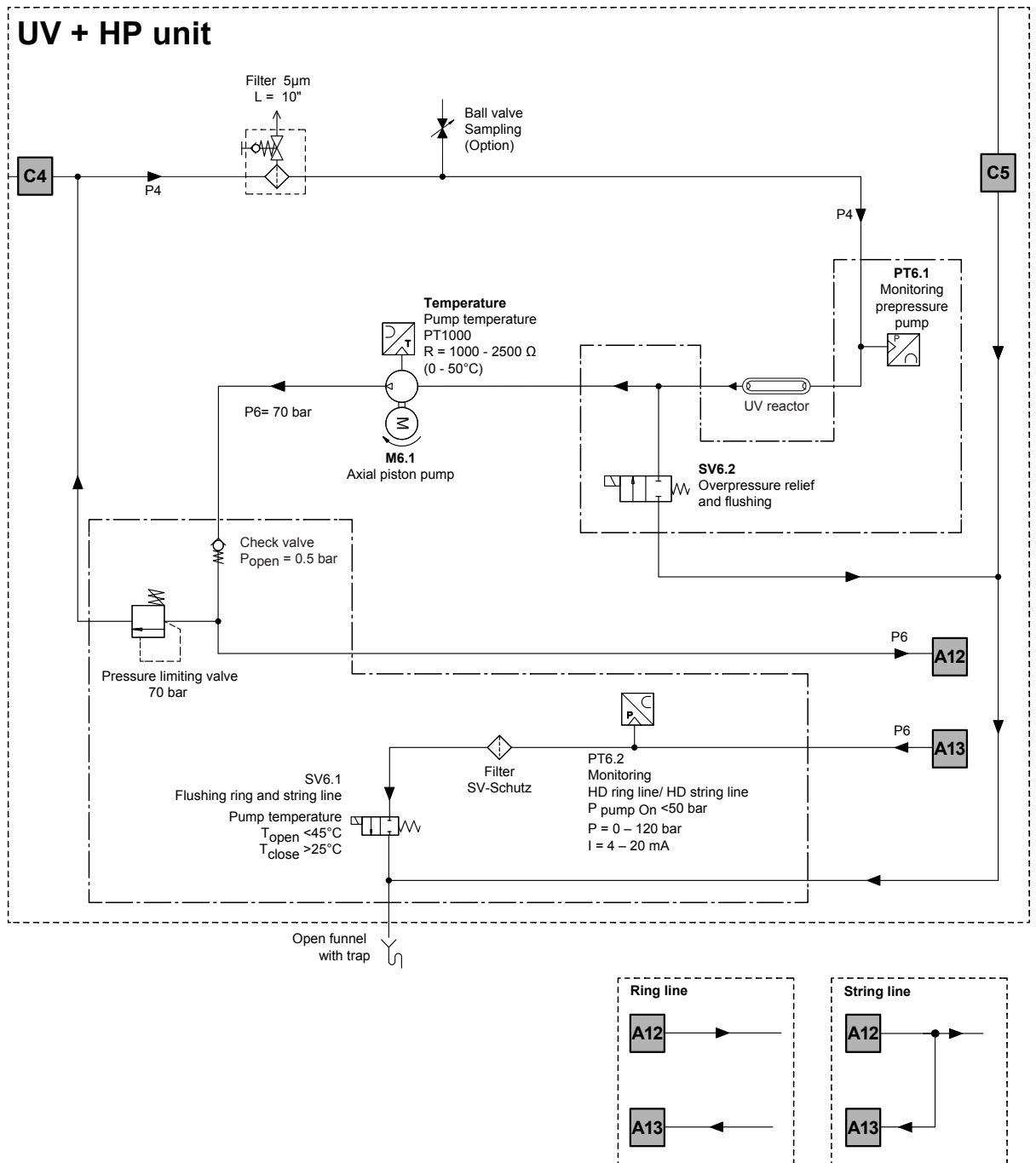
Fig. 25: Hydraulic diagram UV-HP unit
