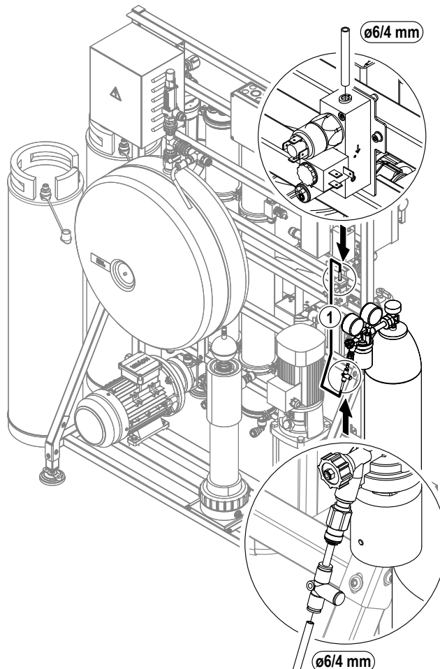
1 JG hose ø6/4 mm / L= 2000 mm (supplied)
