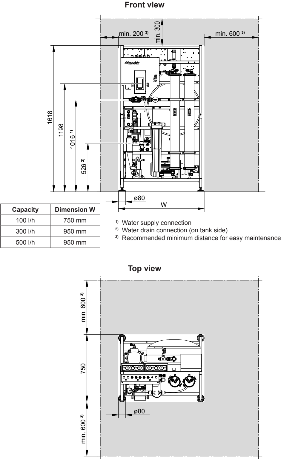
Fig. 6: System dimensions / recommended distances Vita Power RO-UV-HP (dimensions in mm)
