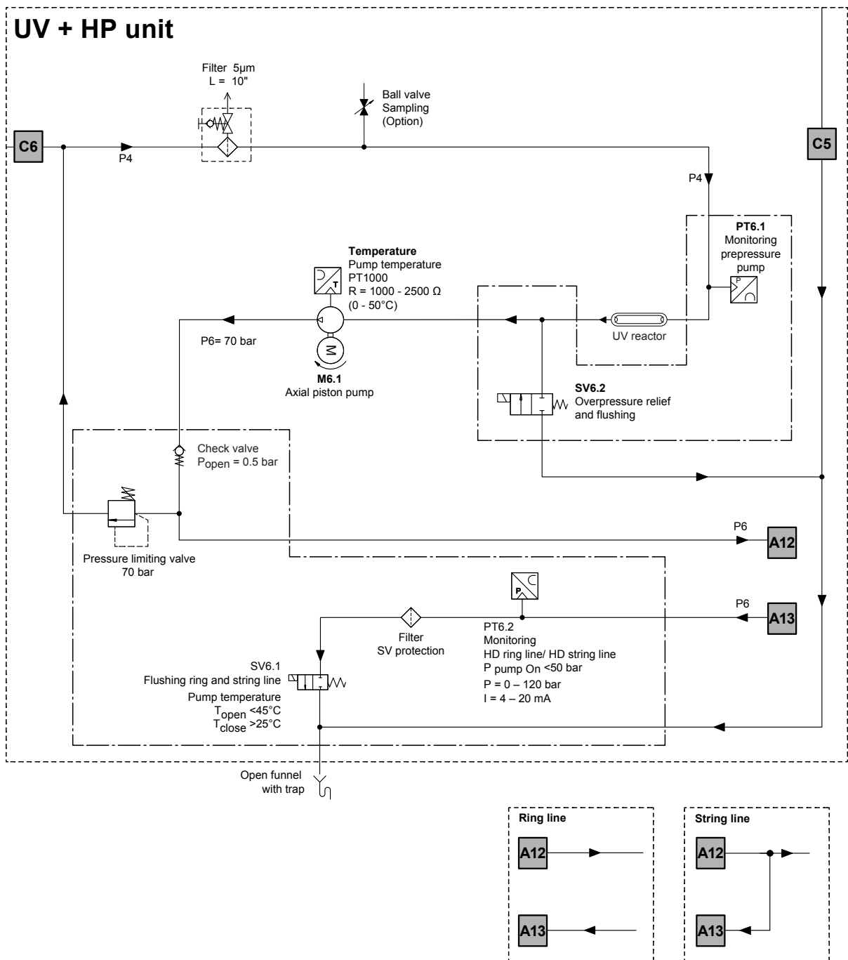
Fig. 22: Hydraulic diagram UV-HP unit
