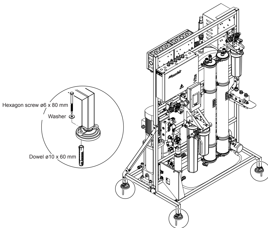
Fig. 9: Mounting of the Condair Vita Power (image shows RO-DI-CO-UV-HP model)
