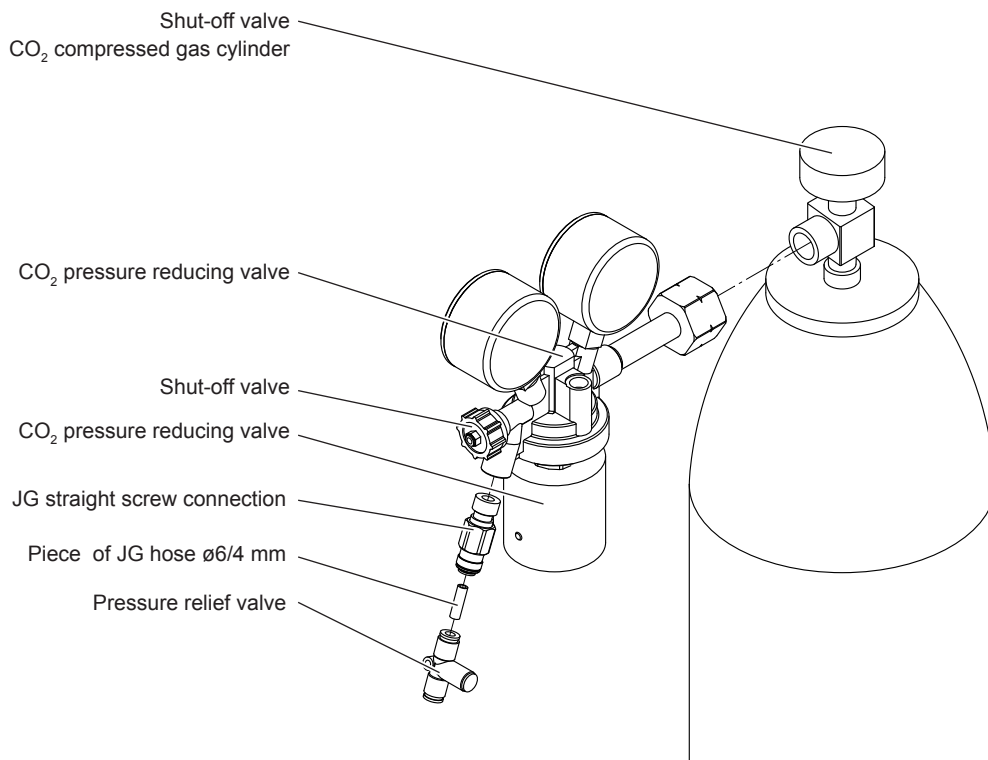
Fig. 16: Connection CO 2 pressure reducing valve
